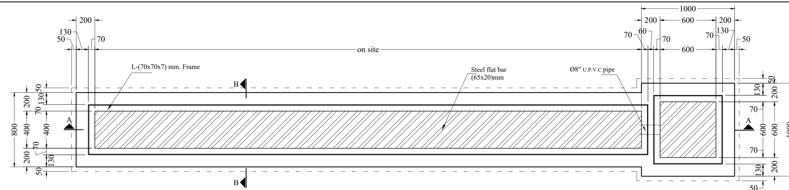
PLAN FOR CATCH BASIN 1:20
