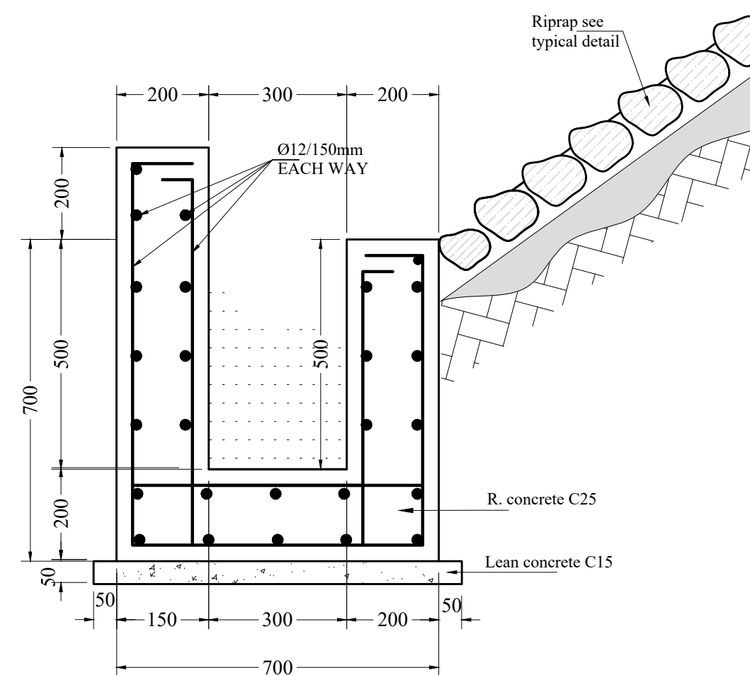
SECTION F-F 1:10
