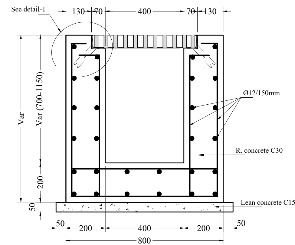
SECTION B-B 1:10
