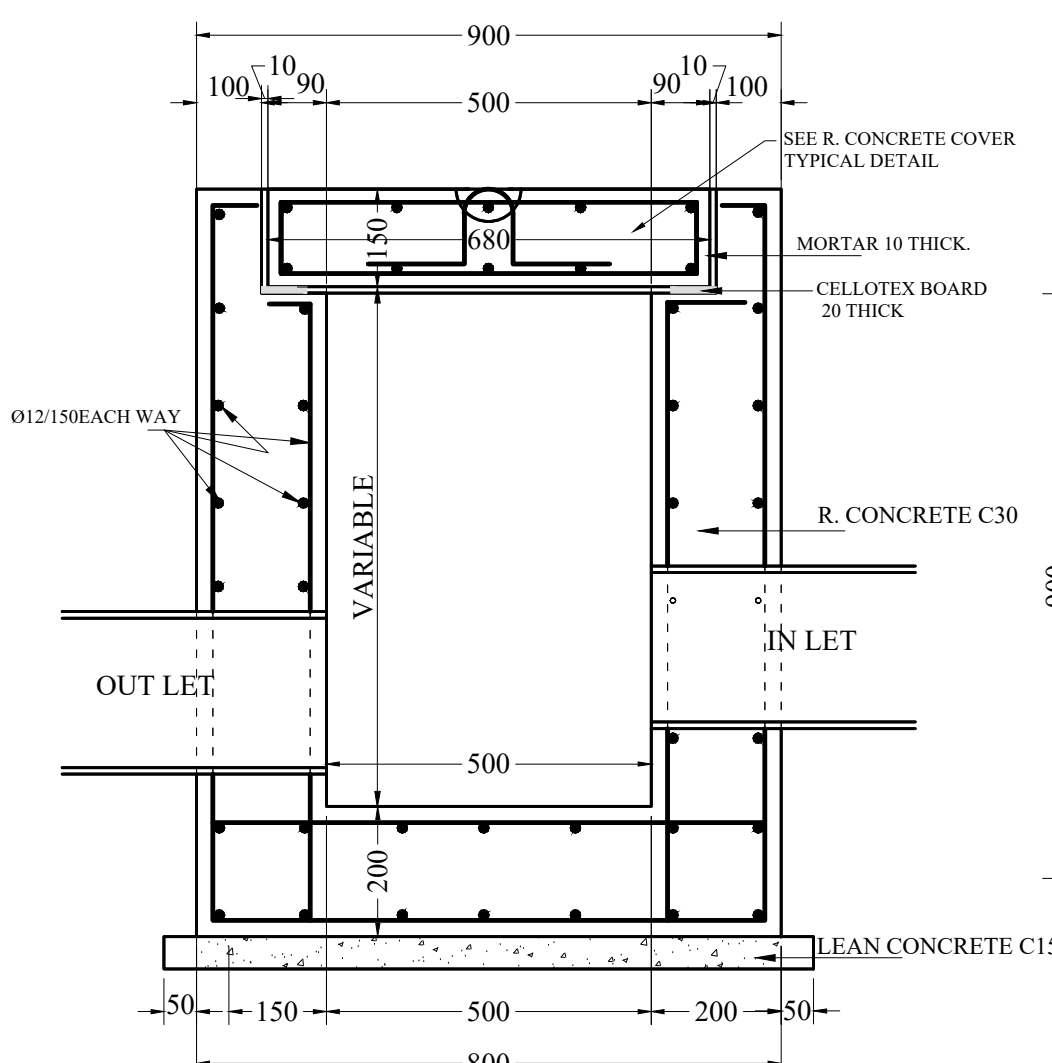
SECTION C-C 1:20
