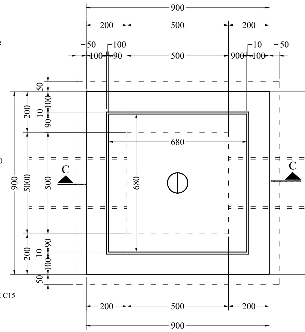
PLAN FOR NEW MANHOLE -MH. 1:10
