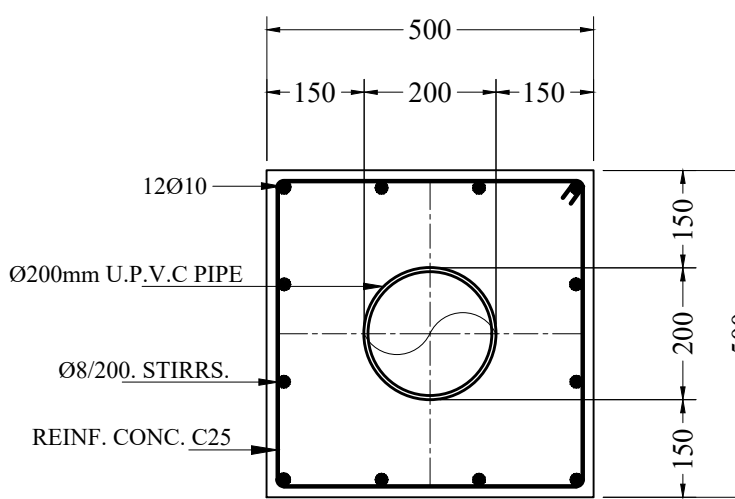
PIPE ENCASEMENT TYPICAL DETAIL 1:5
