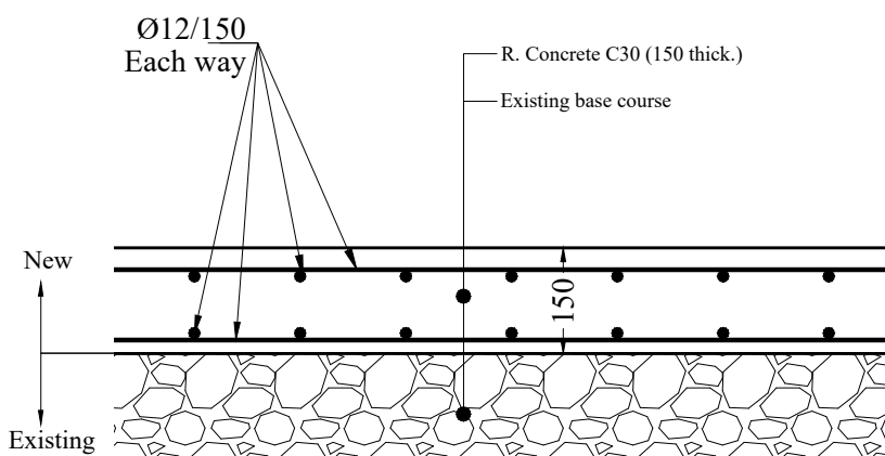
TYPICAL SECTION FOR R. CONCRETE PAVED 1:20
