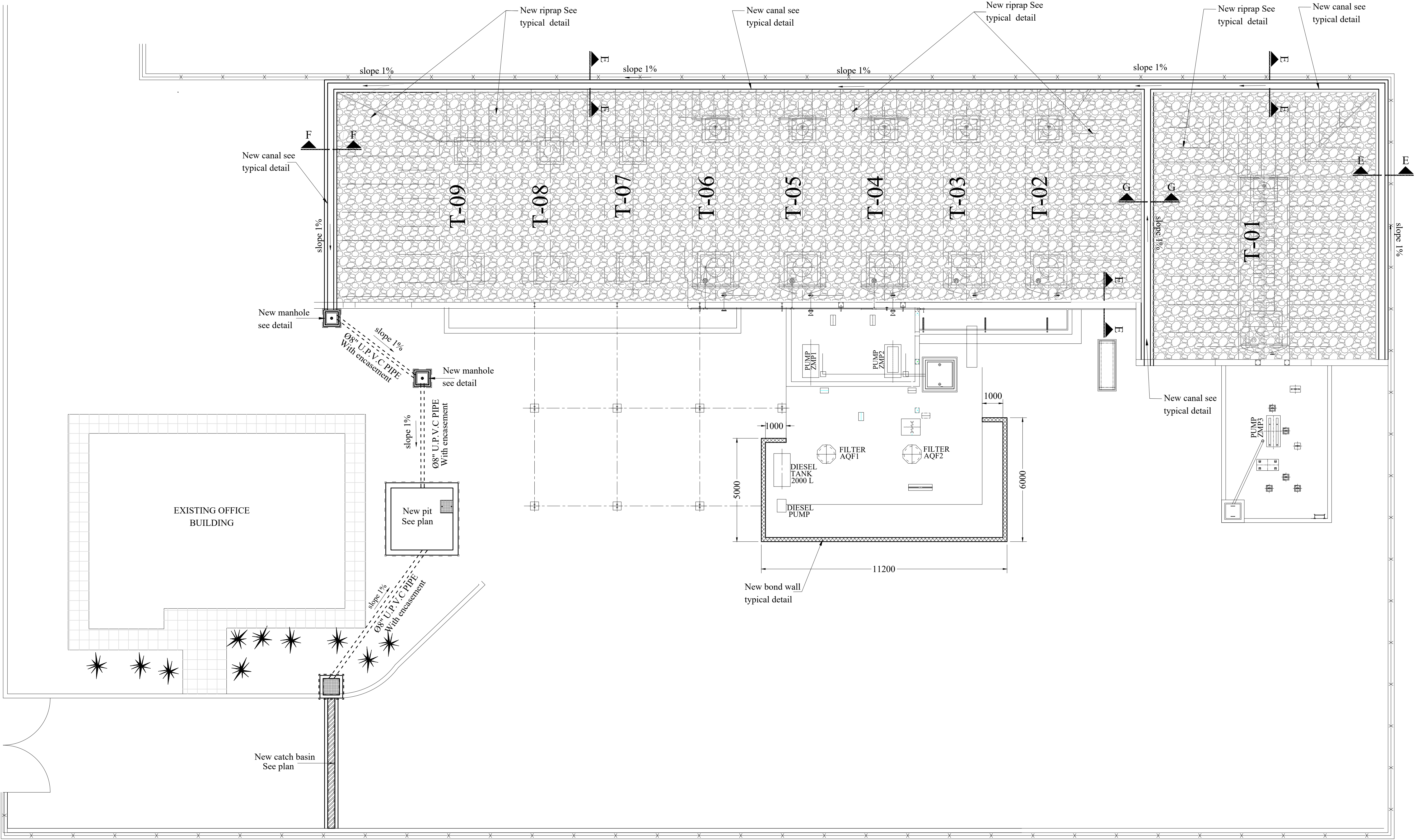
LAYOUT PLAN 1:100
